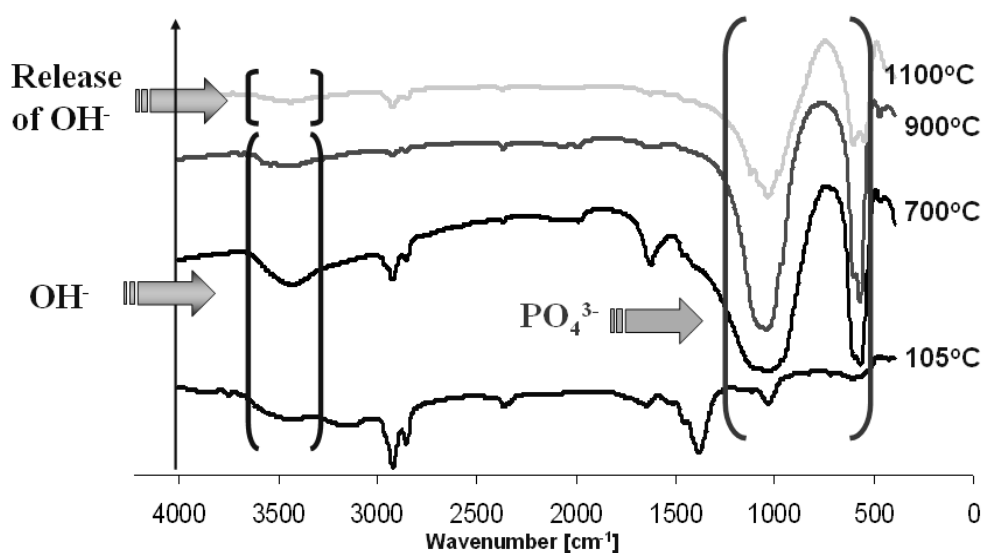
Figure 4. FT-IR spectra of sample II
